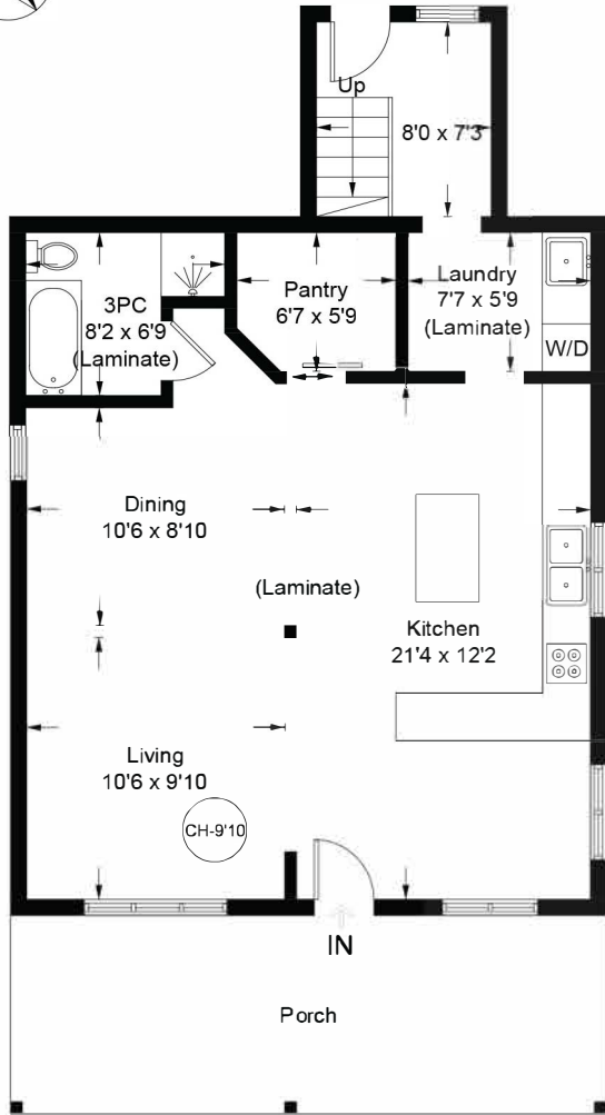
Main Floor - 785 sq ft
