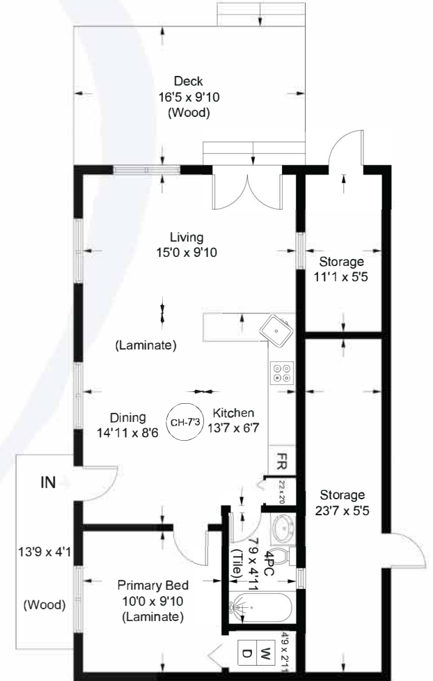
Cabin = 599 sq ft
